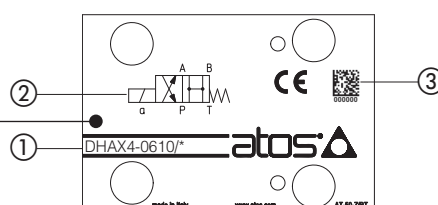
Valve nameplate
