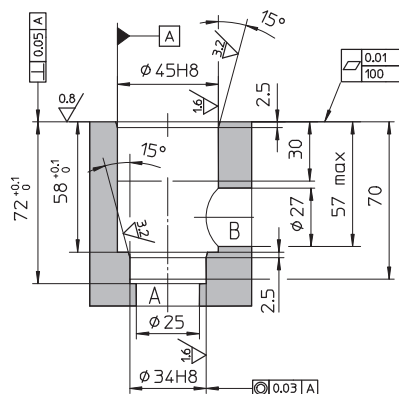
Cavity dimensions for SC LIX-25
