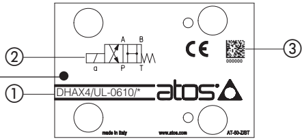
Valve nameplate
