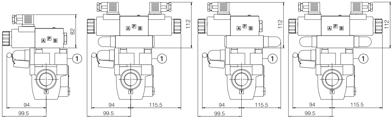
ARAM-20/10/**-EPX ARAM-20/11/**-EPX
