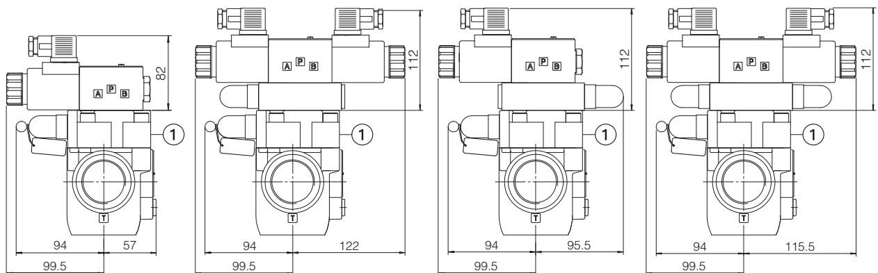
ARAM-32/10/**-EPX ARAM-32/11/**-EPX
