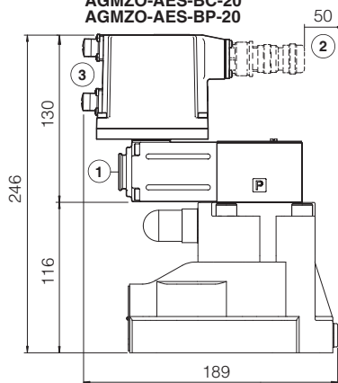
AGMZO-AES-BC-20 AGMZO-AES-BP-20
