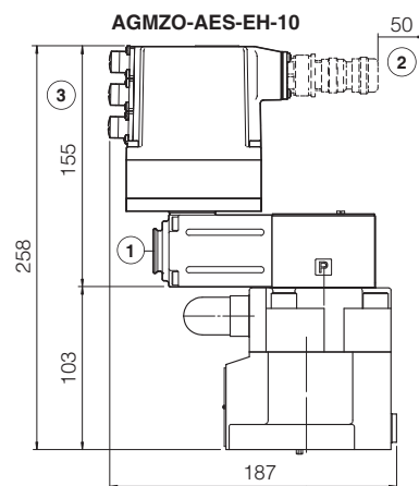
AGMZO-AES-EH-10
