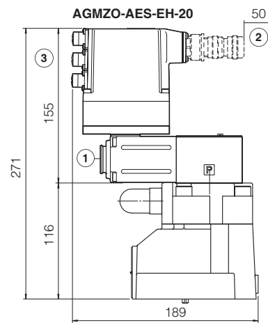
AGMZO-AES-EH-20
