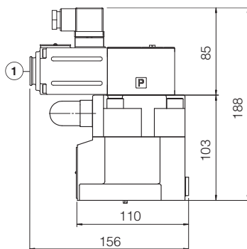
AGMZO-AES-BC-10 AGMZO-AES-BP-10
