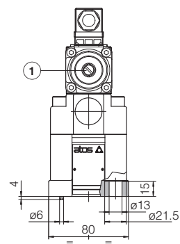
AGMZO-AES-EH-10
