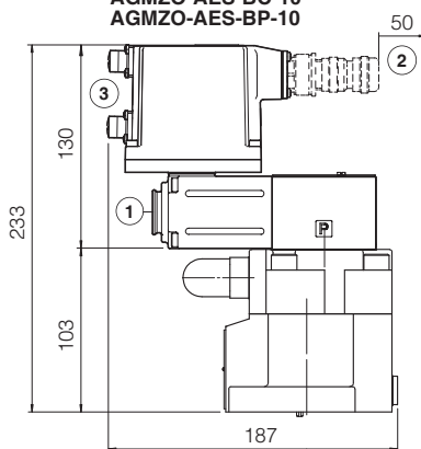
AGMZO-AES-BC-10 AGMZO-AES-BP-10
