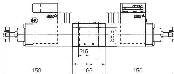
DHAX(S)**-07*/V
