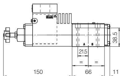
DHAX(S)**-06*/V
