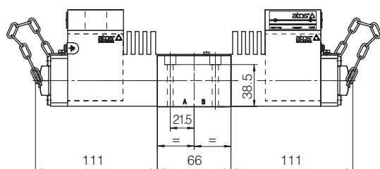
DHAX(S)**-07*
