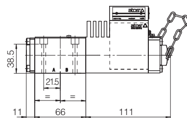
DHAX(S)**-06*/A
