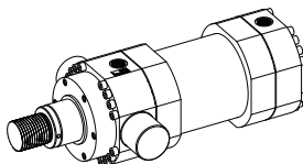
G (ISO MT1) = front trunnion mounting
