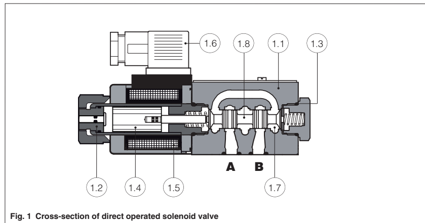
Fig. 1 Cross-section of direct operated solenoid valve
