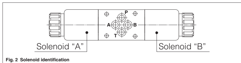
Fig. 2 Solenoid identification
