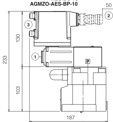
AGMZO-AES-BC-10 AGMZO-AES-BP-10
