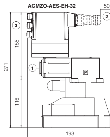
AGMZO-AES-EH-32
