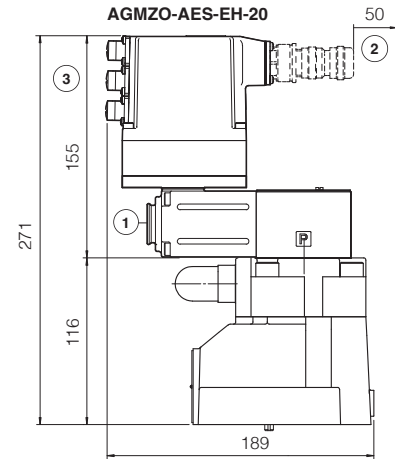
AGMZO-AES-EH-20
