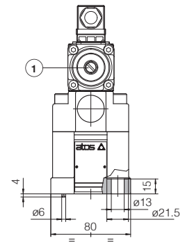
AGMZO-AES-EH-10
