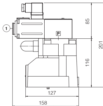
AGMZO-AES-BC-20 AGMZO-AES-BP-20
