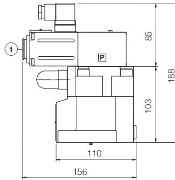
AGMZO-AES-BC-10 AGMZO-AES-BP-10
