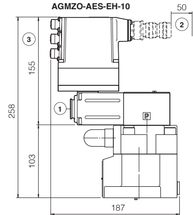
AGMZO-AES-EH-10
